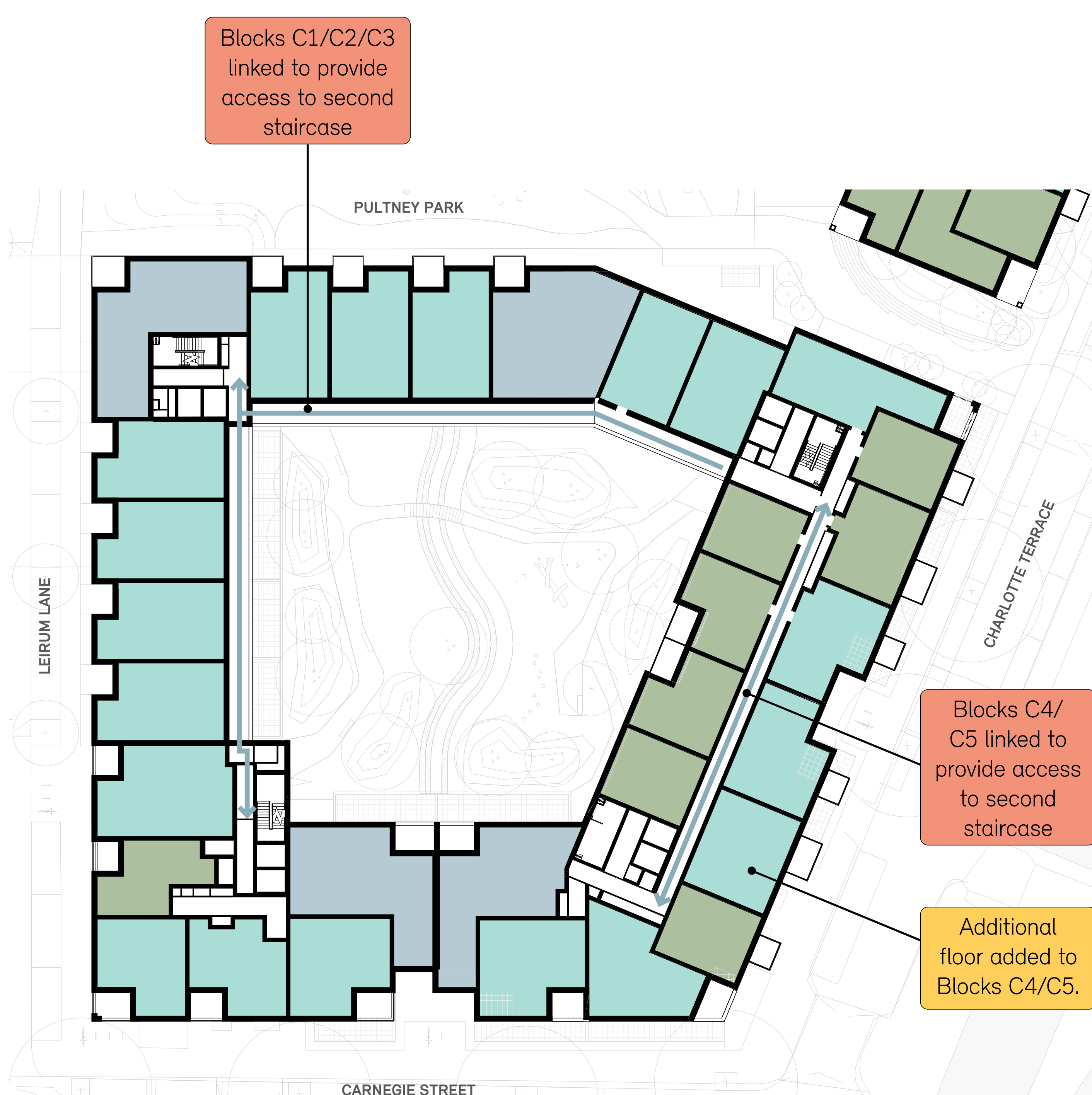
TYPICAL UPPER FLOOR PLAN
